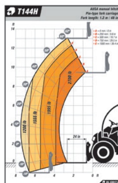
AUSA carriage
